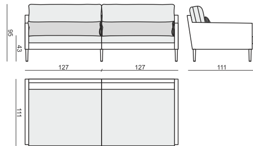
SET 2 DEEP ver. A ELEMENT DEEP LEFT + ELEMENT DEEP RIGHT
